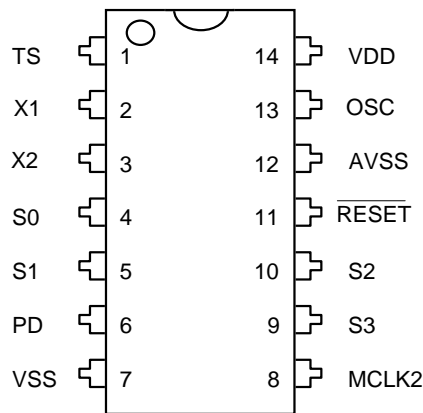
Figure 1: Connection Diagram for Plastic Dip or SOIC Package
