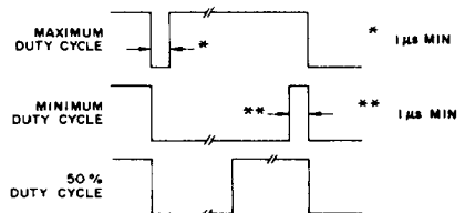
Fig.31 ALLOWABLE TCP, RCP
