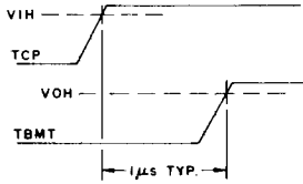
Fig.20 TBMT TURN-ON
