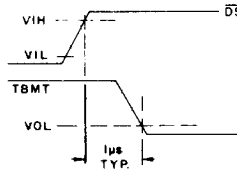
Fig.40 TBMT TURN-OFF
