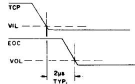
Fig.41 EOC TURN-OFF
