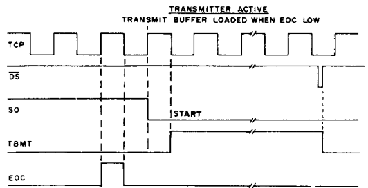
Fig.29 TRANSMITTER AT START BIT
