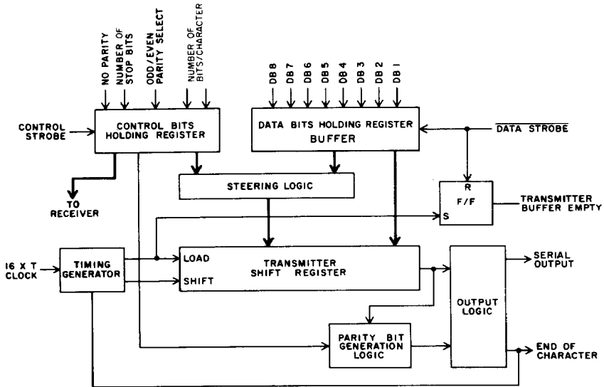
Fig.3 TRANSMITTER BLOCK DIAGRAM
