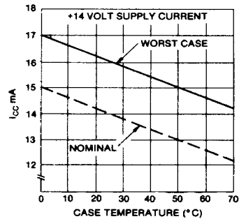
Fig.48 +14 VOLT SUPPLY CURRENT (AY-3-1014A only)
