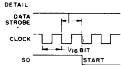
Fig.5 UAR/T TRANSMITTER TIMING
