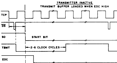
Fig.8 TRANSMITTER AT START BIT
