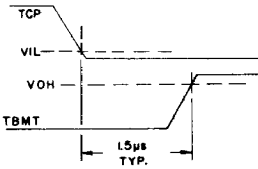
Fig.42 TBMT TURN-ON
