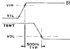
Fig.18 TBMT TURN-OFF
