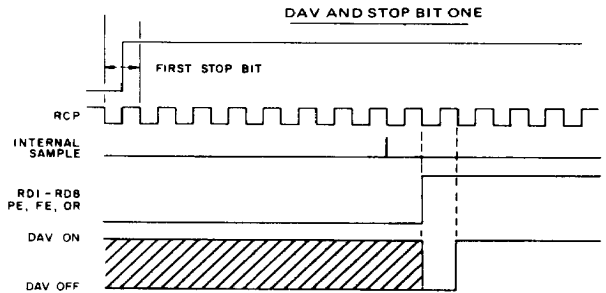
Fig.34 RECEIVER DURING 1ST STOP BIT
