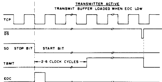
Fig.7 TRANSMITTER AT START BIT
