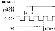
Fig.27 UART — TRANSMITTER TIMING
