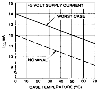
Fig.47 +5 VOLT SUPPLY CURRENT
