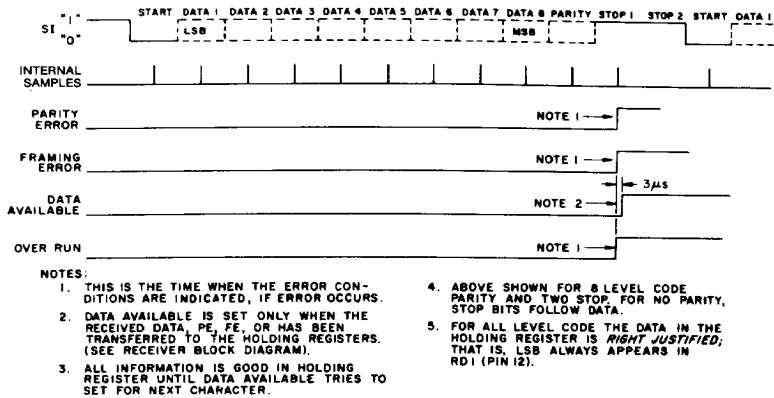
Fig.10 UAR/T RECEIVER TIMING
