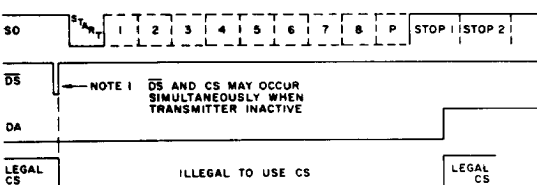
Fig.8 ALLOWABLE POINTS TO USE CONTROL STROBE
