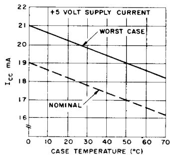
Fig.26 +5 VOLT SUPPLY CURRENT
