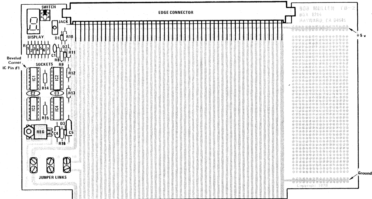
Parts Placement Diagram
