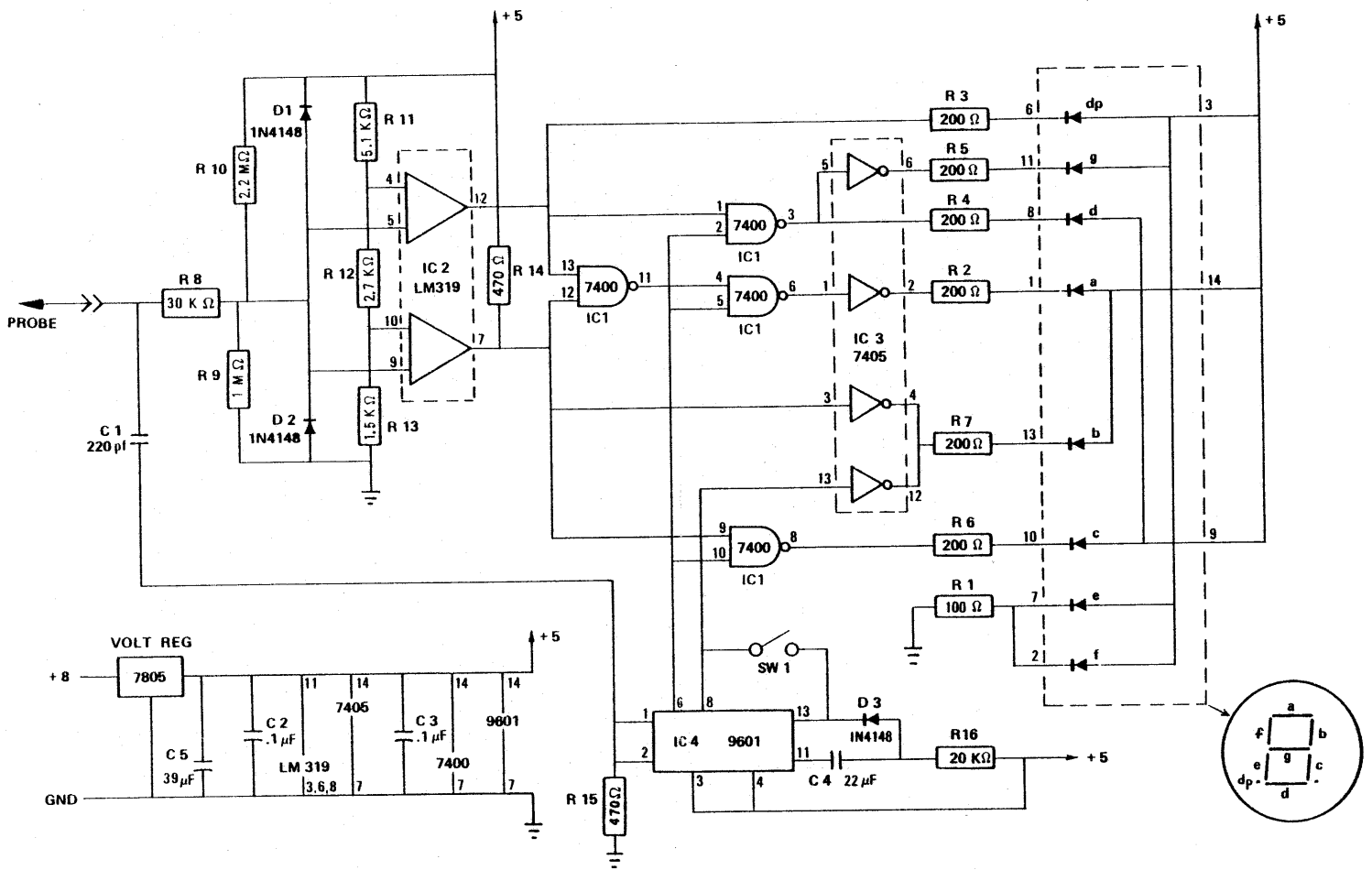
SCHMATIC FOR LOGIC PROBE
